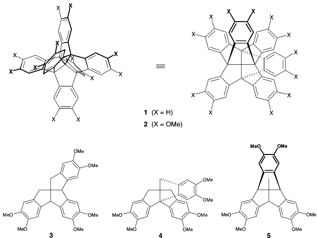
Scheme 1. Centrohexasindanes 1 and 2 and the veratrole-type centrotriindanes 3–5 . The latter three formulae are presented strictly as cuttings of the right-hand formula of 2 .
