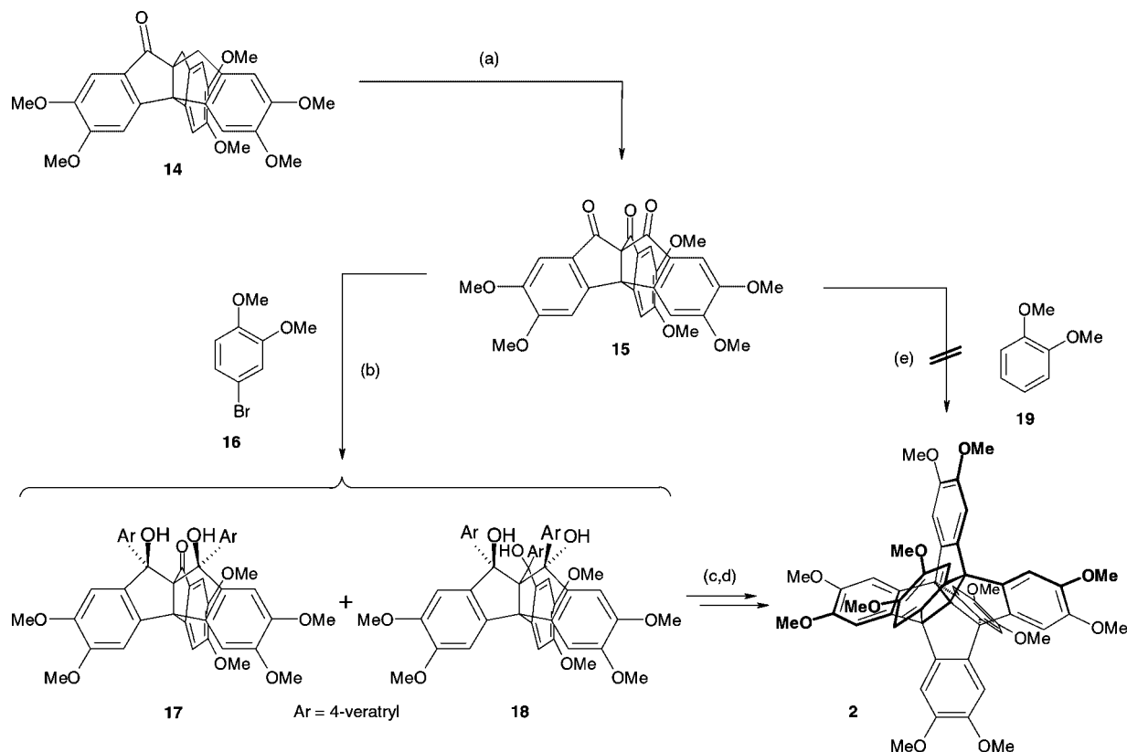
Scheme 4. (a) \text{CrO}_3 , \text{AcOH}/\text{H}_2\text{O} , 20^\circ\text{C} , 24 h, 27%; (b) 1. Mg, THF, 16 , \Delta , 4 h; 2. benzene, 20^\circ\text{C} , 16 h; (c) 1. \text{H}_3\text{PO}_4 (85%), chlorobenzene, \Delta , 2 h; 2. NaH, \text{CH}_3\text{I} , THF, \Delta , 18 h, 6%; (e) see Exp. Sect..
